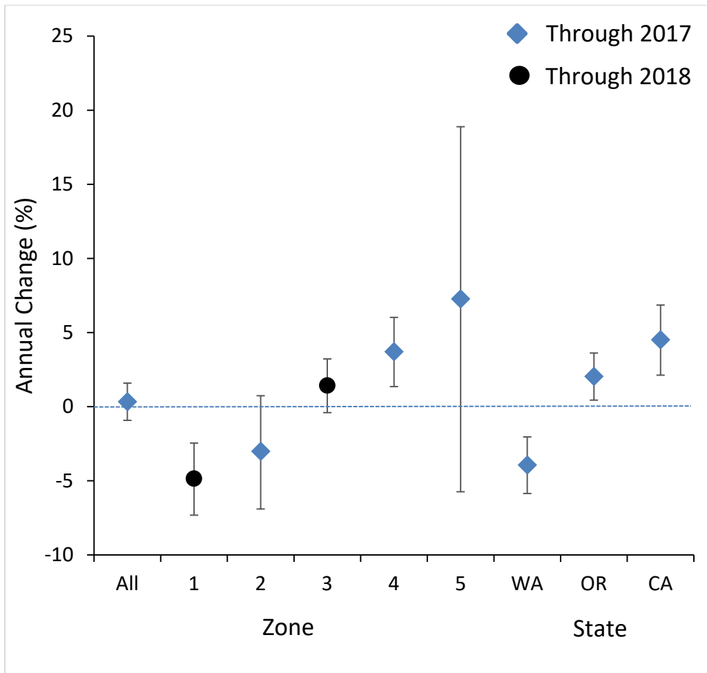
Figure 2. Percent annual change (95% Confidence interval) by Conservation Zone, “All”-Zones combined and by State. Trends are through 2017 for the blue squares and through 2018 for the black circles. If the confidence intervals do not overlap zero, then there is support for either a positive (e.g., Zone 4) or a negative (e.g., Zone 1) trend. Note that these results are provided in a tabular form in Table 2.
