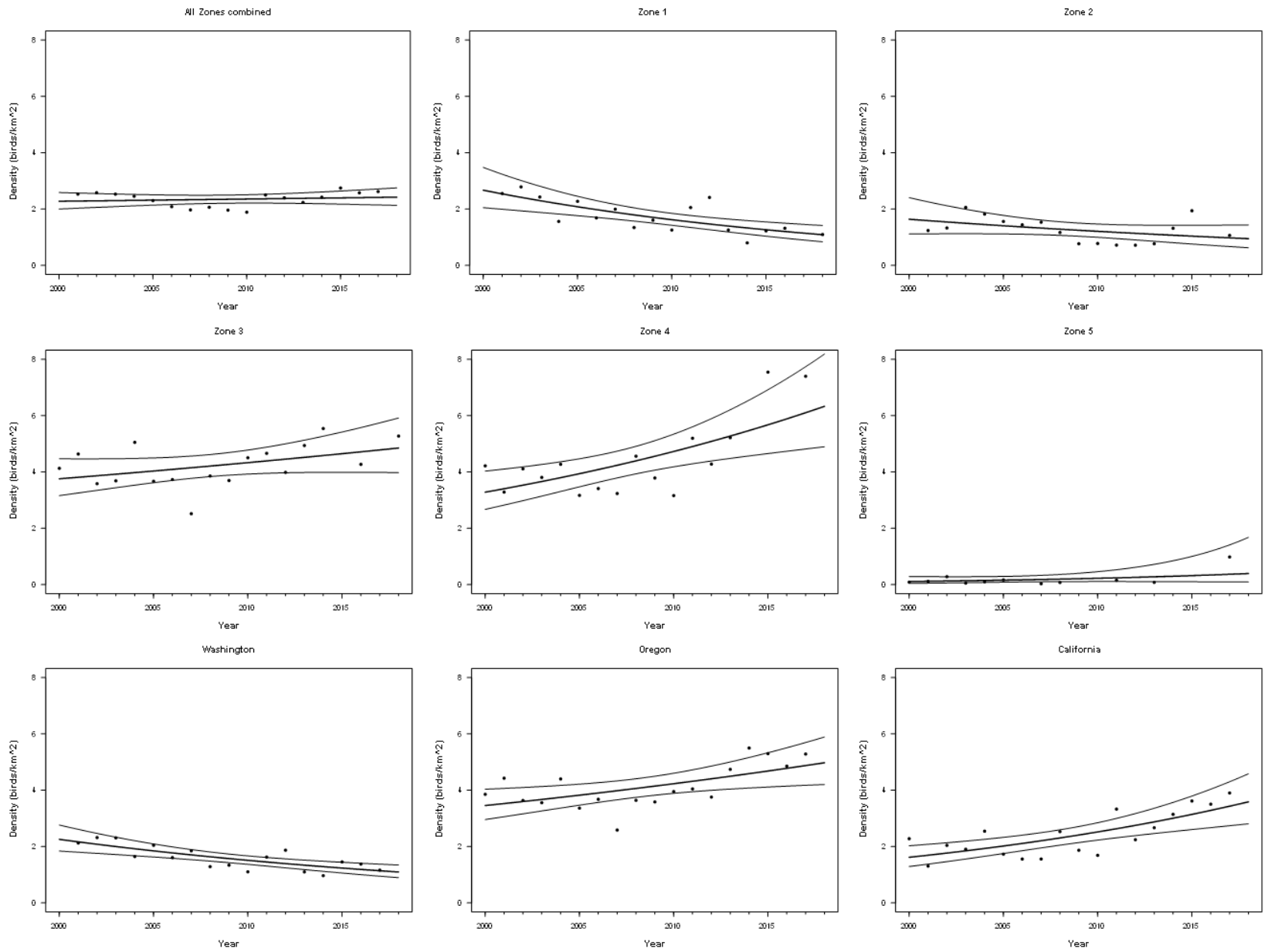
Figure 3. Marbled murrelet population trend analyses for All-Zones, individual Conservation Zones, and State scales. Graphs show fitted regression lines through the annual population estimates for the period of analysis (through 2017 for Zones 2, 4, and 5 only), with 95 percent confidence limits.
